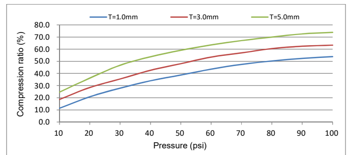
Compression Ratio
