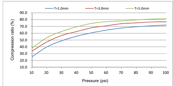
Compression Ratio
