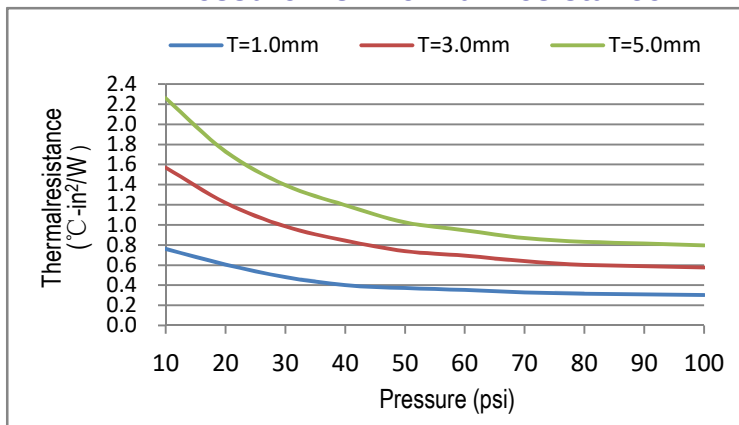
Pressure. vs. Thermal Resistance
