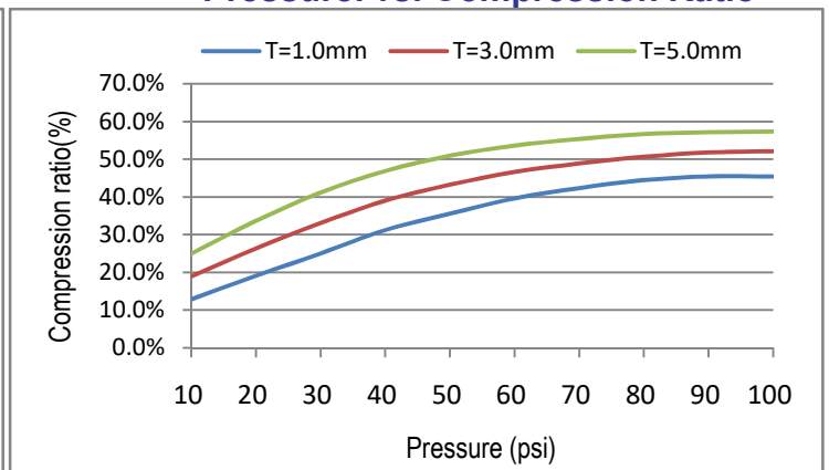
Pressure. vs. Compression Ratio
