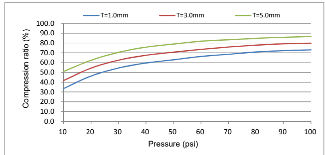
Compression Ratio
